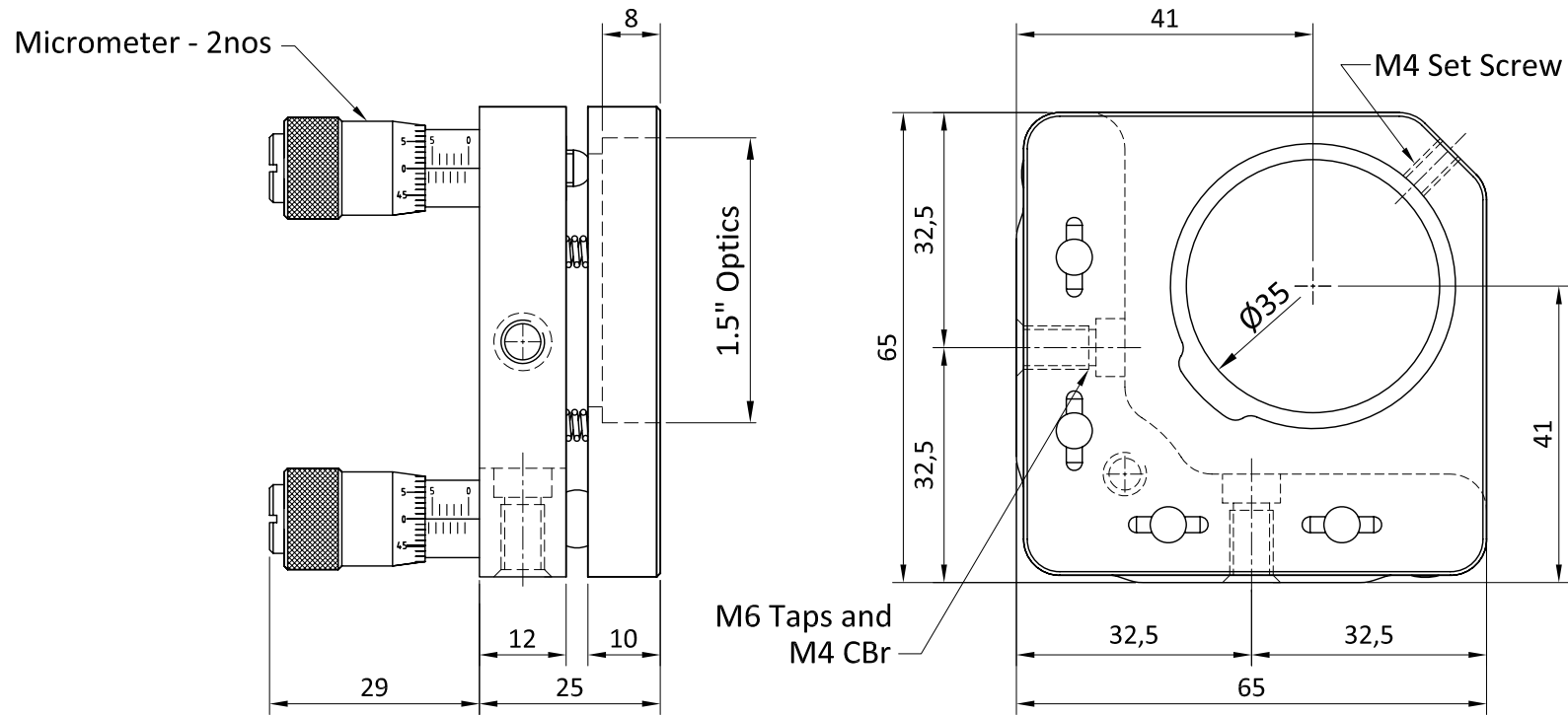
1.5" or 38mm optic mount
