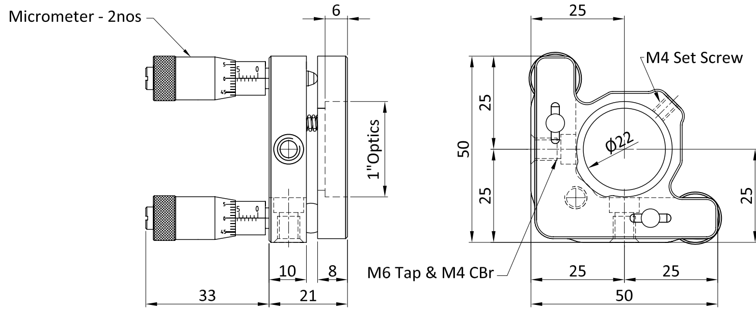
1" or 25mm optic mount
