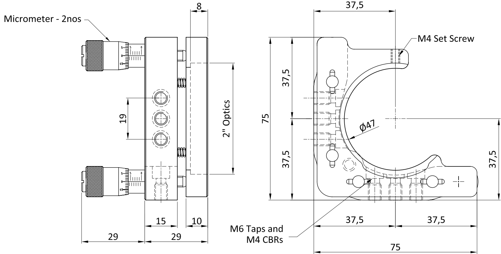
2" or 50mm optic mount
